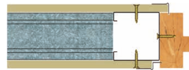
DETAIL A: DOOR/WINDOW HEAD DETAIL
