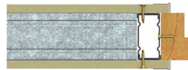
FIGURE 6: INTERNAL WALL FRAMING
