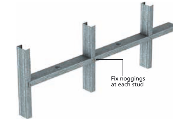
FIGURE 7: STANDARD NOGGING TRACK DETAILS
