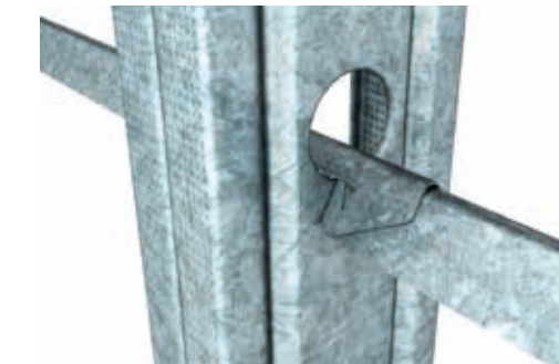
FIGURE 8: OVERLAPPING OF SNAP-LOCK NOGGING® WHEN CONTINUOUS
