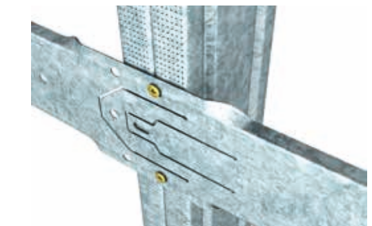
FIGURE 11: FAST-FIX NOGGING® INSTALLED INTO RONDO STEEL STUD USING FACE-FIX x 2 SCREWS METHOD
