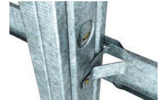
FIGURE 10: BACK VIEW OF TAB/FACE FIX x 3 SCREWS INSTALLATION METHOD
