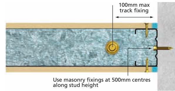
FIGURE 1: INTERSECTION - MASONRY
