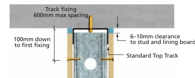
FIGURE 5: FRICTION FIT APPLICATION
