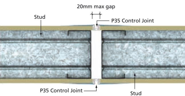
FIGURE 3: STUD WALL CONSTRUCTION WITH CONTROL JOINT
